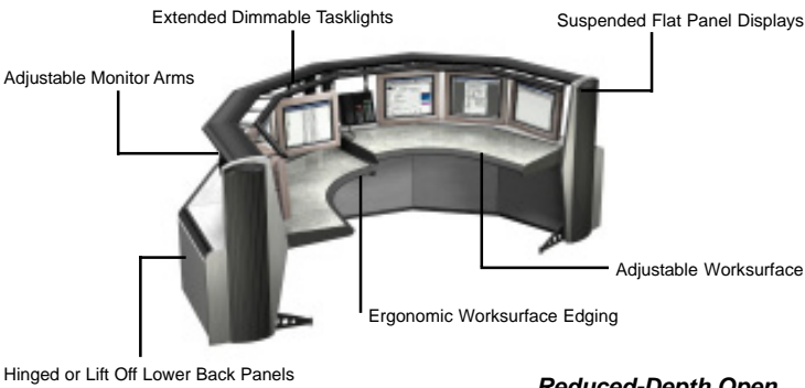
Reduced-Depth Open
